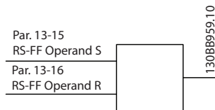
Illustration 3.55 Bascules Reset-Set
