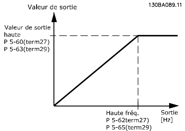
Illustration 3.40 Configuration des sorties impulsions
