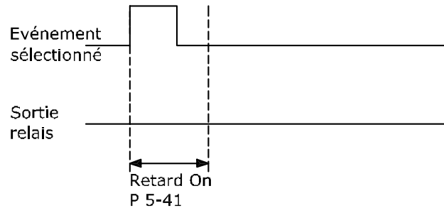
Illustration 3.37 Relais, retard ON
