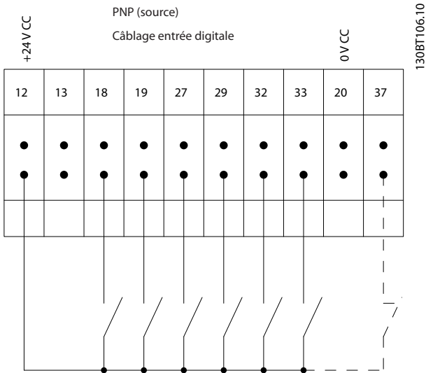
Illustration 1.3 PNP (source)
